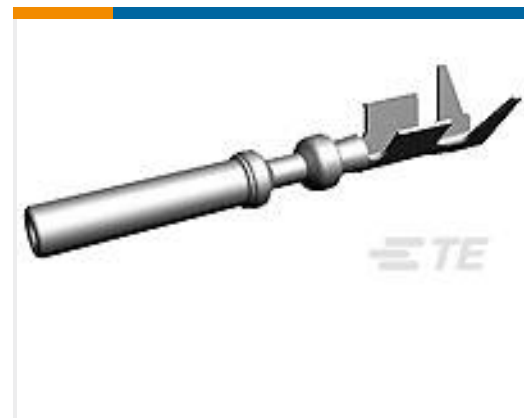
TE Part #3-1447221-3 S/S REC CONTACT ASSY, AU, 0.75~1.25
