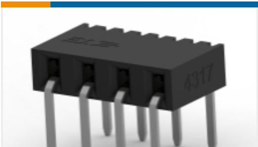
TE Part #2314938-4 4P,2MM,B-B,REC,SRHZ,2.8,0.76AU,TR
