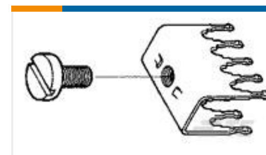
TE Part #5055323-5 06 PWR TAP CONT PLTD STD .125
