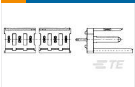
TE Part #280609-2 2P MOD 1 SHROUDED HEADER, ST, 0.4 Au
