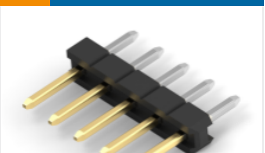
TE Part #2355186-5 5P,2MM,BRK HDR,SRVT,2.8,0.76AU, BOX
