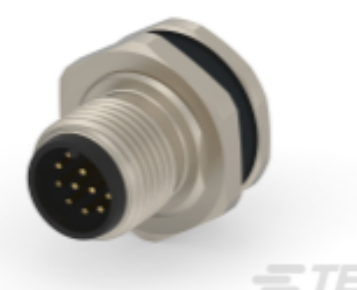
TE Part #T4171030012-001 M12,REAR MOUNT,MALE, A, 12P, 0.2 M WIRE
