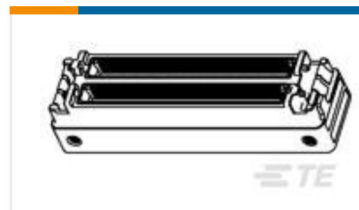
TE Part #1775470-2 HPI CONN., 2.0MM, V/T, SMT, 2P, 80U"
