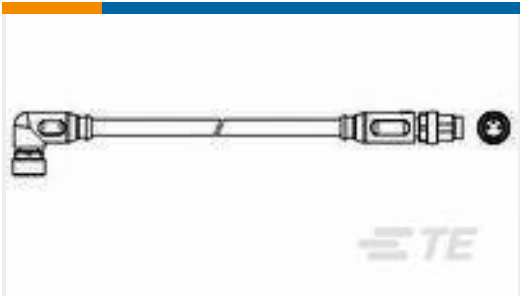
TE Part #1-2273124-5 M8 angled socket to M8 straight plug 2 LED
