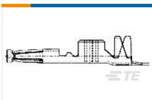
TE Part #1719532-1 MQS0,63 Sn rec CB unseal. AWG18
