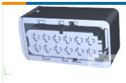
TE Part #1-1670901-1 12POS,AMP MCP2.8,REC HSG,ASSY
