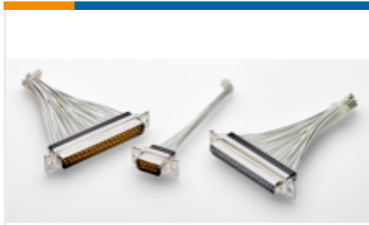
TE Part #2335893-4 AMPLIMITE SZ 4 RECPT 62 POS, ST STL SHEL
