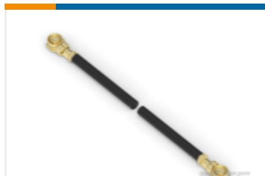
TE Part #1-2016698-3 UMCC CA, GEN4-GEN4,1.13,L150MM, BK
