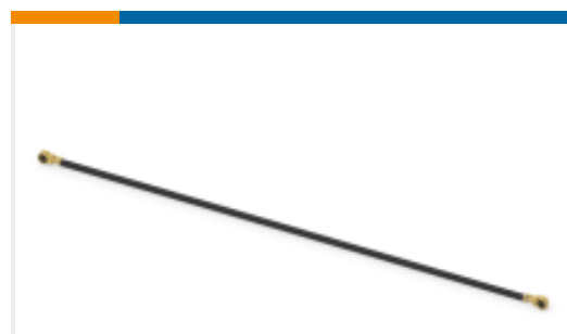
TE Part #1-2016698-2 RF CA,UMCC GEN4-GEN4,1.13MM CABLE,L100MM
