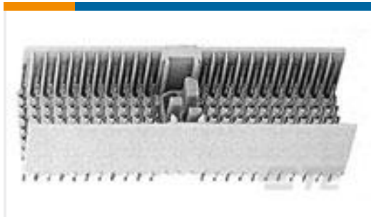
TE Part #188834-1 Z-PACK/A M-HDR 154P.
