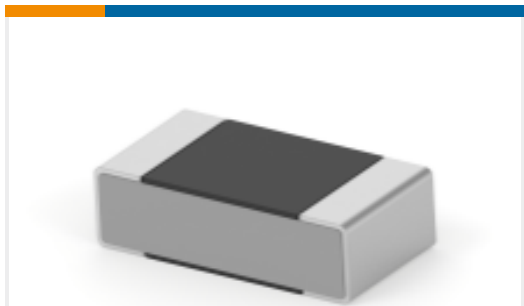
TE Part #5-1879207-4 RN 0603 357K 0.1% 10PPM 5K RL
