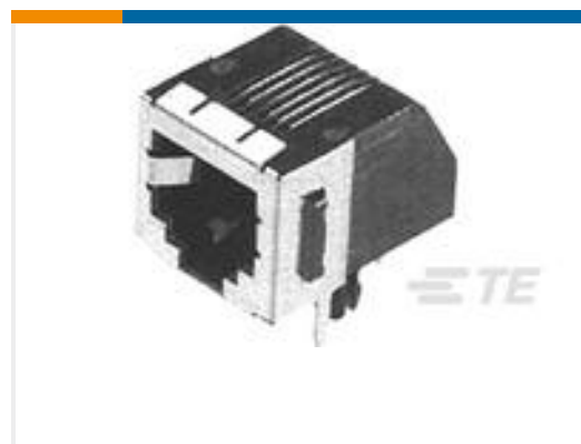
TE Part #5555140-1 MJ,LPF,R/A,6P/6C,SHLD,PNL GRD
