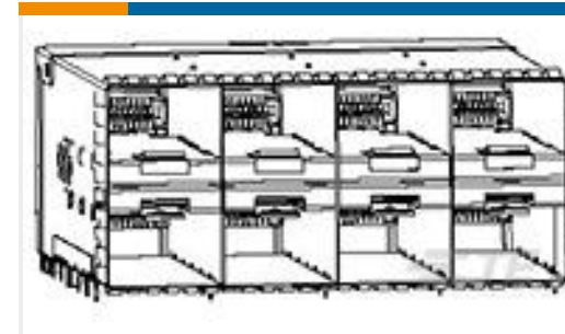
TE Part #1-2180324-9 zSFP+ STACKED 2X4 RECEPTACLE ASSEMBLY
