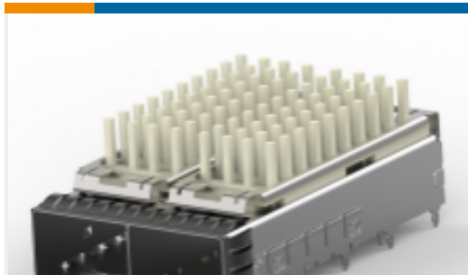
TE Part # 2198230-3 SFP+ Enhanced 1x2, Networking Heatsink
