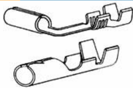
TE Part #42142-2 SHUR PLUG TERMINAL 18-14 AWG BR
