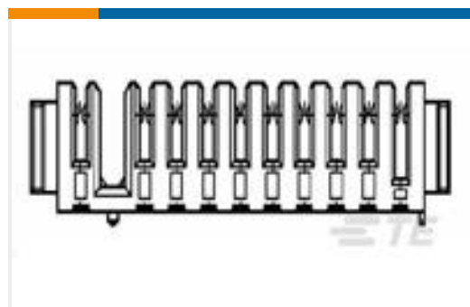
TE Part #1-1473776-7 2.5MM PITCH BATTERY REC ASSEMBLY SMT TYP
