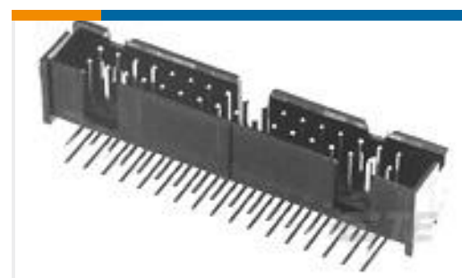
TE Part #5103310-1 A/L LOW PRO HDR 10P RA BLACK
