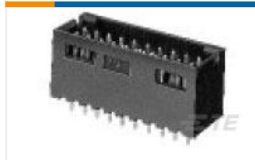
TE Part #8-87589-5 08 MODII HDR DRST SHRD .100CL
