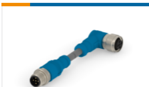
TE Part #T4162124005-001 RPC-M12-5MS-0.5SH-M12-5FR-PUR
