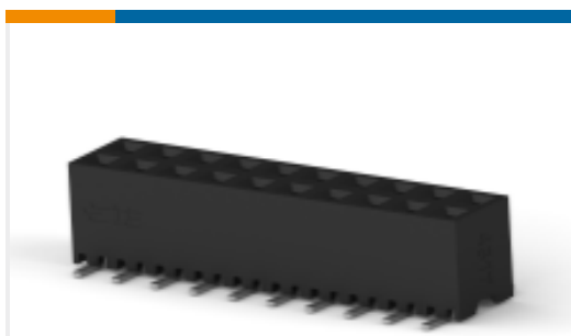
TE Part #2-2314844-0 20P, 2MM, B-B, REC, DRVT, SMD, 0.1AU, TB, W/CP
