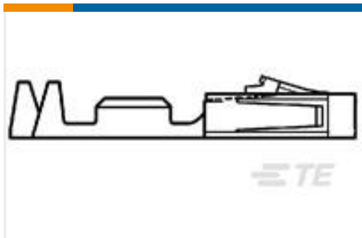
TE Part #1-104481-2 SHORT POINT RECP CONT LP
