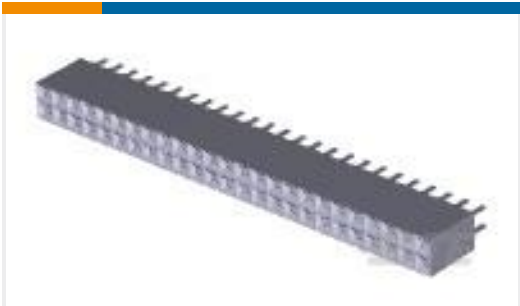
TE Part #7-534206-5 50 MODII VRT DR CE 100/115
