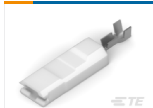
TE Part #520974-2 ULTRA POD: Straight, Receptacle Assembly, Tin Plated, 0.25 inch
