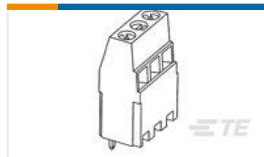
TE Part #1-282901-2 TERM-BLK PCB MT 2ND 12P.5.08,
