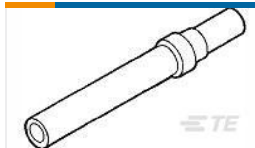
TE Part #1218267-1 CONT,CRIMP SKT,18AWG,109,SZ 20
