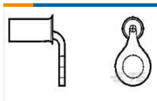
TE Part #35625 TERMINAL,SOLIS R 90DEG 4 1/4
