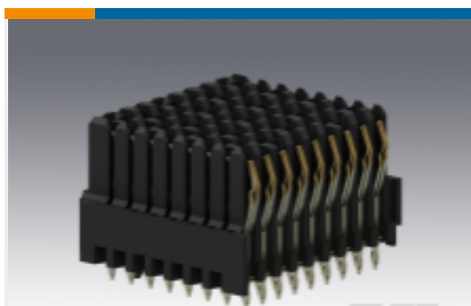
TE Part #2102735-2 Assy, Vert Recpt, Left End, MG, Rug Cntc
