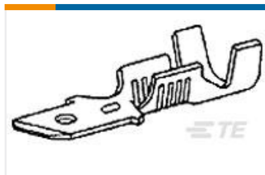
TE Part #42490-3 187 FASTON TAB 22-18 AWG TPBR
