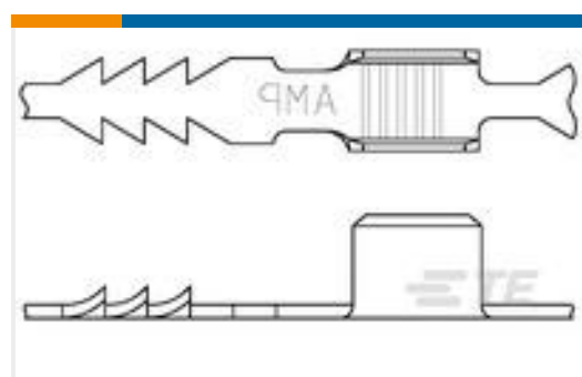
TE Part #62192-1 BOBBIN TAB .016TPBR
