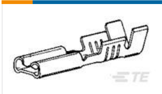
TE Part #160626-1 110 FASTON,REC.,20-17 AWG,BR
