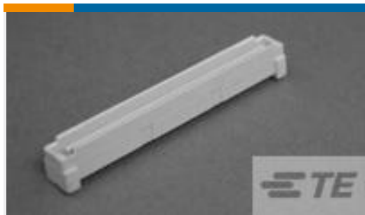
TE Part #5179030-1 0.8FH,P07H.5,040,08/Sn,TU
