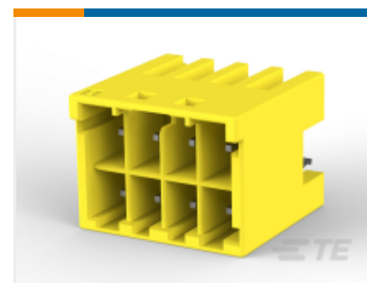
TE Part # 4-1971906-4 HEADER ASSY 8POS,KEYING-D,NEW GIC3.3
