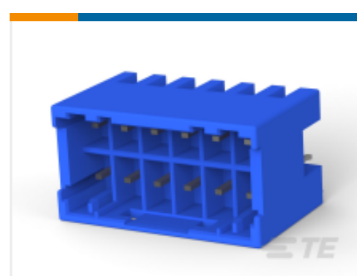
TE Part # 2-1871571-3 GIC 3.3 HEADER ASSY 12POS
