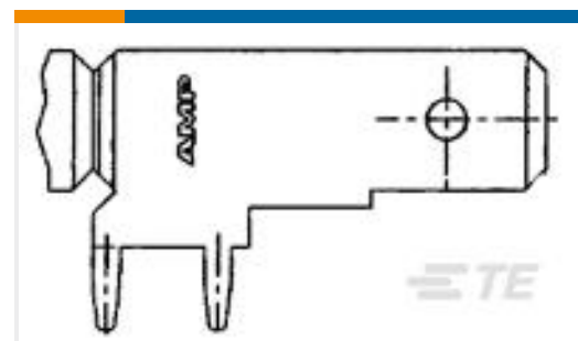
TE Part #63407-2 PL 187 TERMINAL REC 0.2-0.5 MM2 PTPBR
