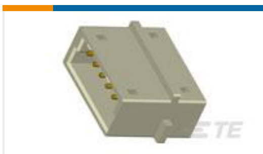
TE Part #292156-2 CT RELAY HDR ASSY FREE HANGING
