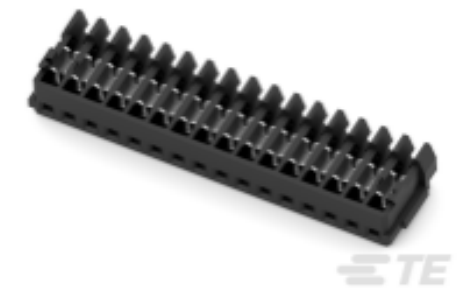
TE Part #3-353293-6 1.5MM CT MT REC ASSY 16P BLACK
