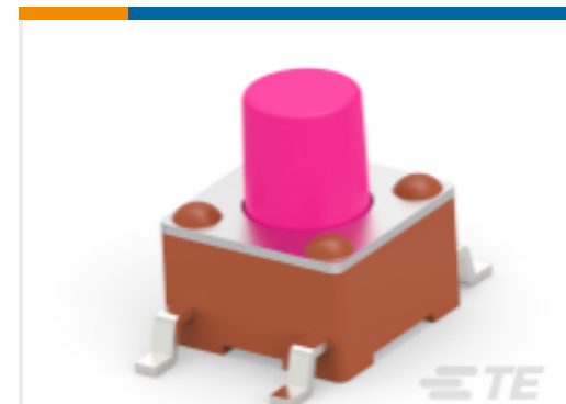
TE Part #1-1977223-9 FSM6JSMAAS=6MM TACT SWITCH, SMT 260gf
