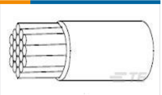
TE Part #080443-000 22759/44-12-9
