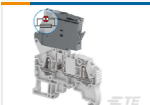
TE Part #1SNK706411R0000 ZK2.5-SF-R1
