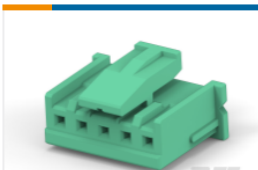
TE Part #8-2338183-5 EP 2.5 HOUSING 5P, GREEN, UL version
