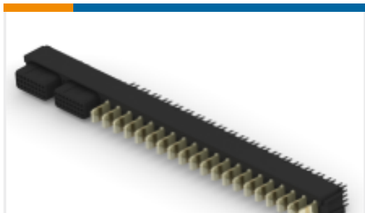
TE Part #6646272-1 CONN,SKT,STR,COMPL,FLATPAQ
