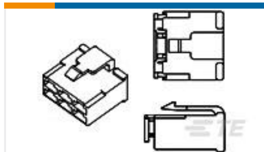
TE Part #6437288-2 SUPERSEAL Connector Headers: 1.0 mm
