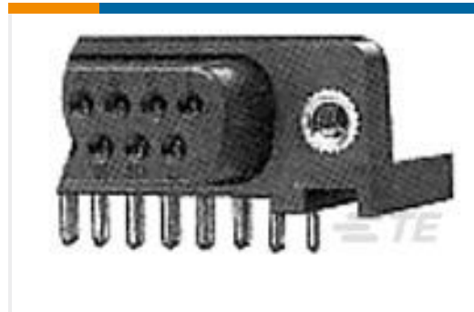
TE Part #5788796-1 09 HTMSFL ASSY RA 318 (IN,BL)
