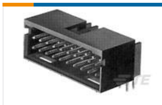
TE Part #6-102617-3 30 MODII HDR DRRA SHRD LF
