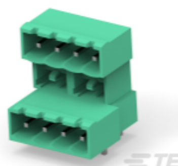
TE Part # 284061-6 TERMI-BLOK HDR 90, 5,08MM P. M
