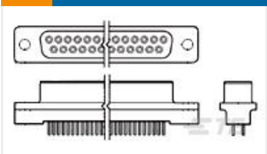
TE Part #5207841-3 HD-20 RCPT 9P VERT THD INS
