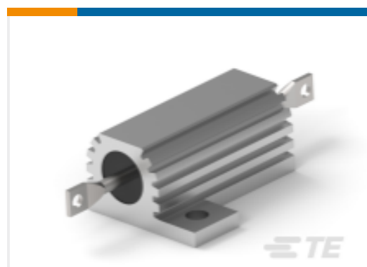
TE Part #3-1879075-0 Power Resistor: Aluminum Housed, 75 Watt
