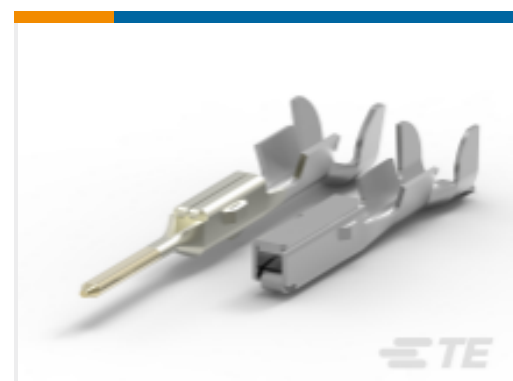
TE Part #173645-3 MULTILOCK, RECEPTACLE AND TAB
