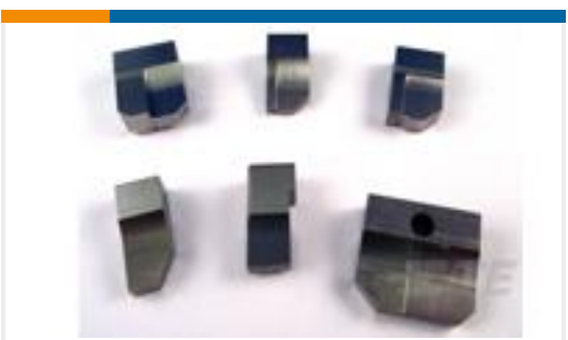
TE Part #1376348-1 5MM POWER KEY CONN REC CONT M
