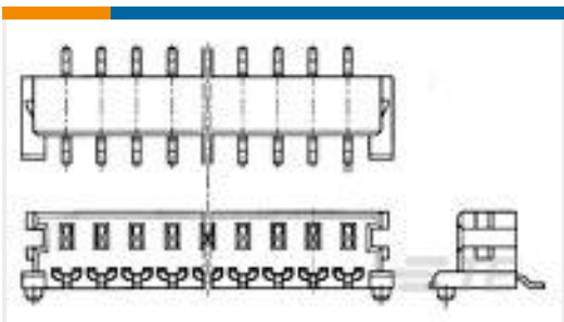
TE Part #8-917570-7 1.5 WTB HDR ASSY 7P AU-TYPE
